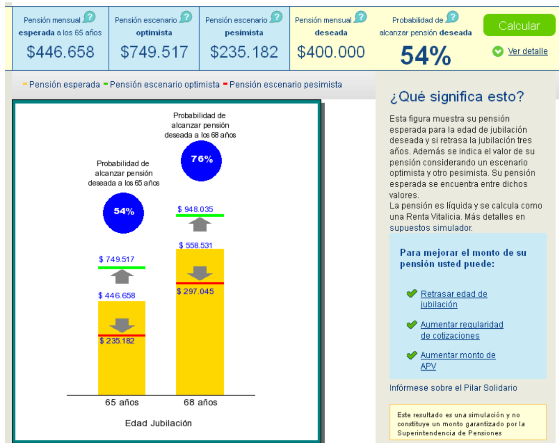
Figure 10: Simulator Outputs
